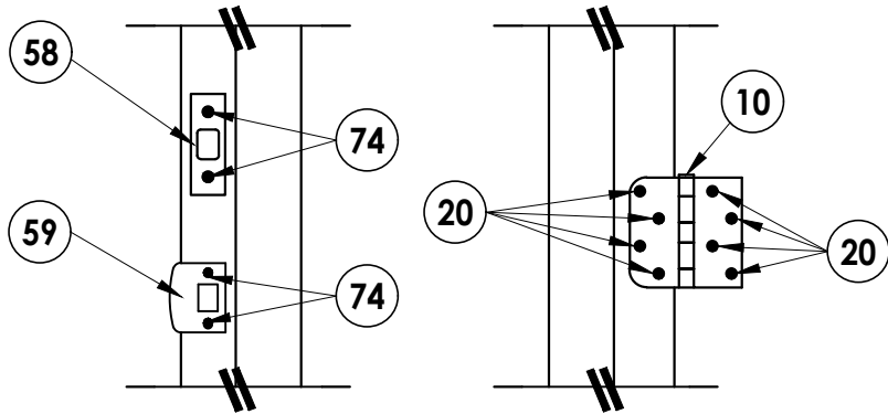
STRIKE PLATE DETAIL
