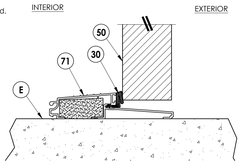
2 VERTICAL CROSS SECTION 5 Shown w/ Outswing Threshold
