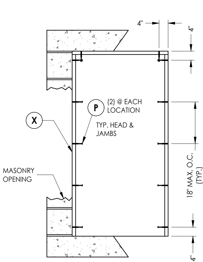
BUCK ANCHORING Masonry steel stud construction
