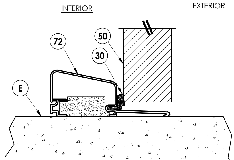
3 VERTICAL CROSS SECTION 5 Shown w/ High Dam Threshold
